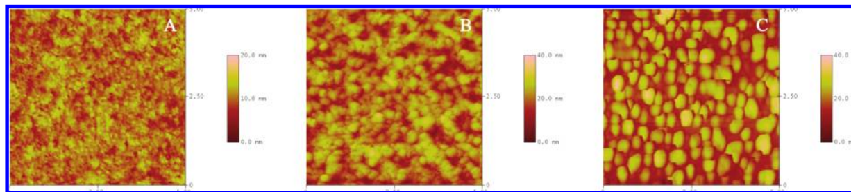
Figure 5. AFM topography images of the two 10-layer compound 1 films at room temperature deposited on bare SiO 2 /Si substrate (scan range: 5 × 5 μm 2 ; height: 0–20 nm; tapping mode) (A), HMDS-treated SiO 2 /Si substrate (scan range: 5 × 5 μm 2 ; height: 0–40 nm; tapping mode) (B), and OTS-treated SiO 2 /Si substrate (scan range: 5 × 5 μm 2 ; height: 0–40 nm; tapping mode) (C).
