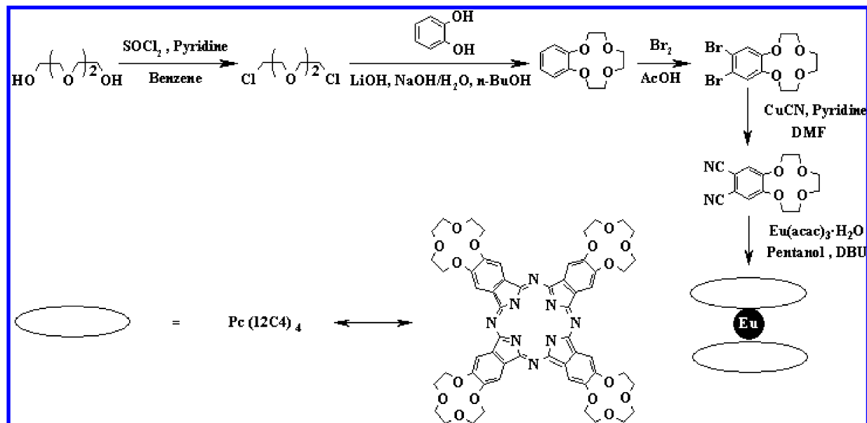
Scheme 2. Synthesis of 4,5-Di(12-crown-4)phthalonitrile and Homoleptic Bis[2,3,9,10,16,17,23,24-tetrakis(12-crown-4)phthalocyaninato] Europium Complex
